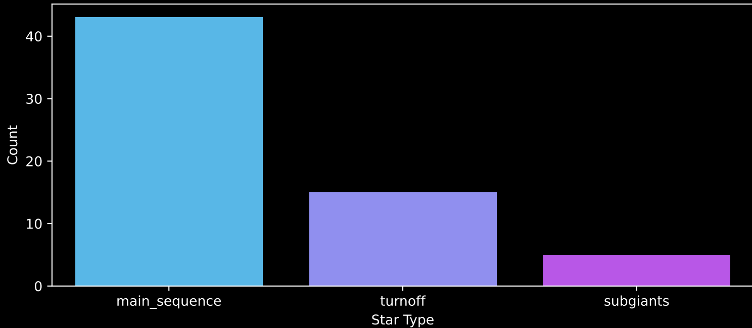
APOGEE DR17 Field: [209-20-C] Count plot of Star Type
