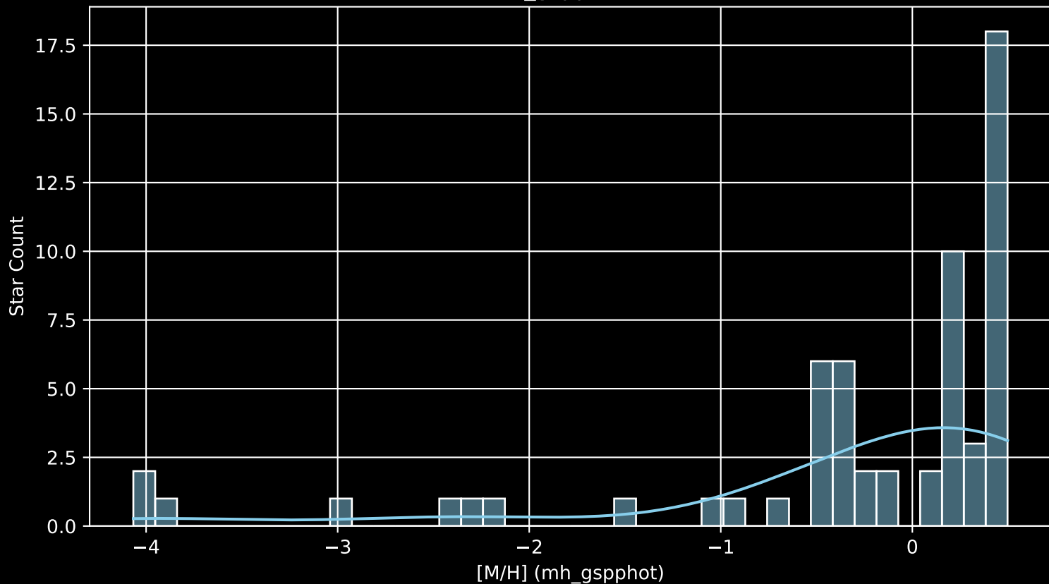
APOGEE DR17 Field: [209-20-C [M/H] (mh_gspphot) (n= 60)
