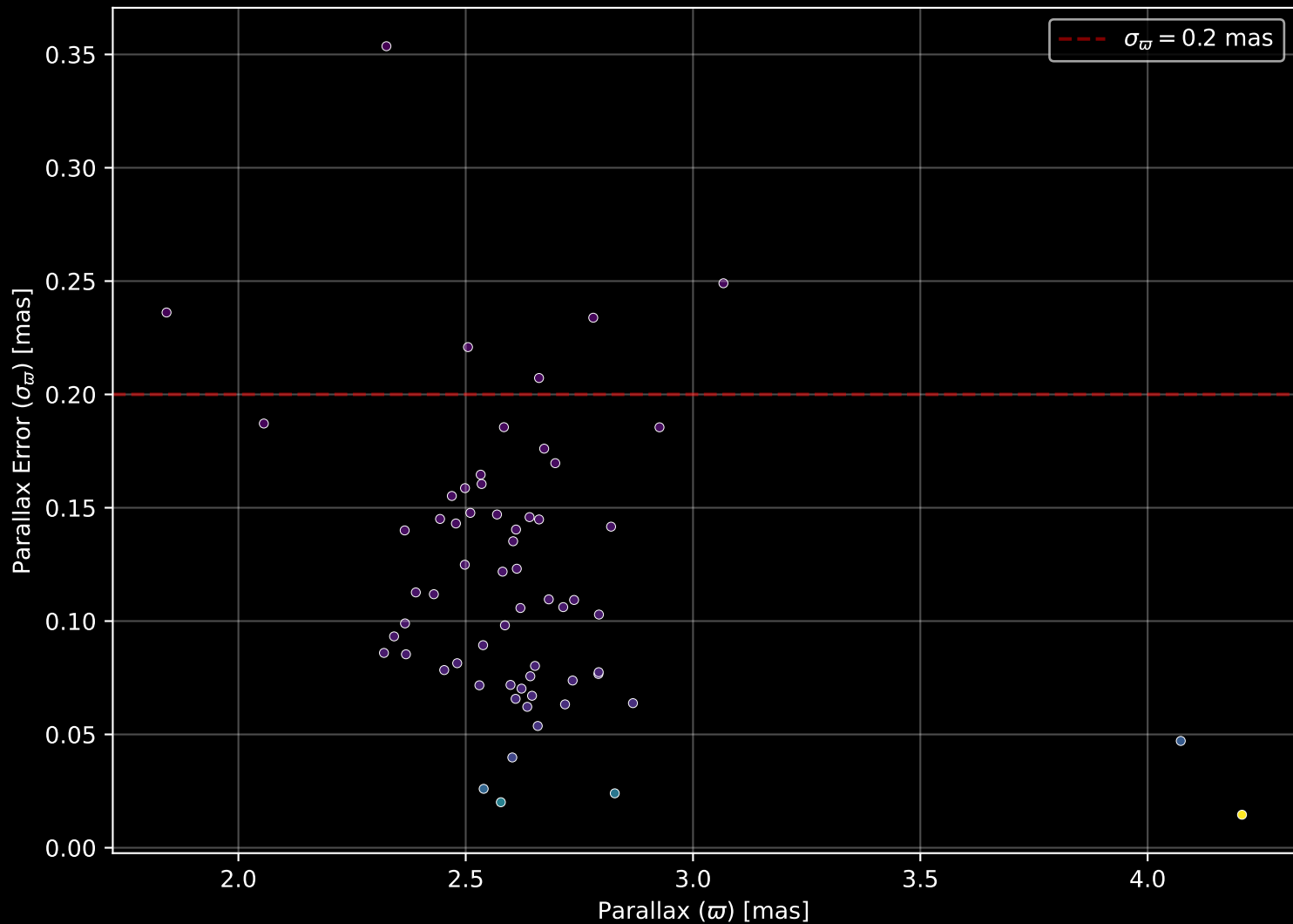
APOGEE DR17 Field: [209-20-C] Parallax Quality (n= 63)
