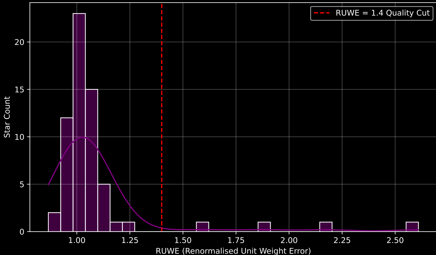
GAPOGEE DR17 Field [209-20-C] RUWE Distribution (n= 63)
