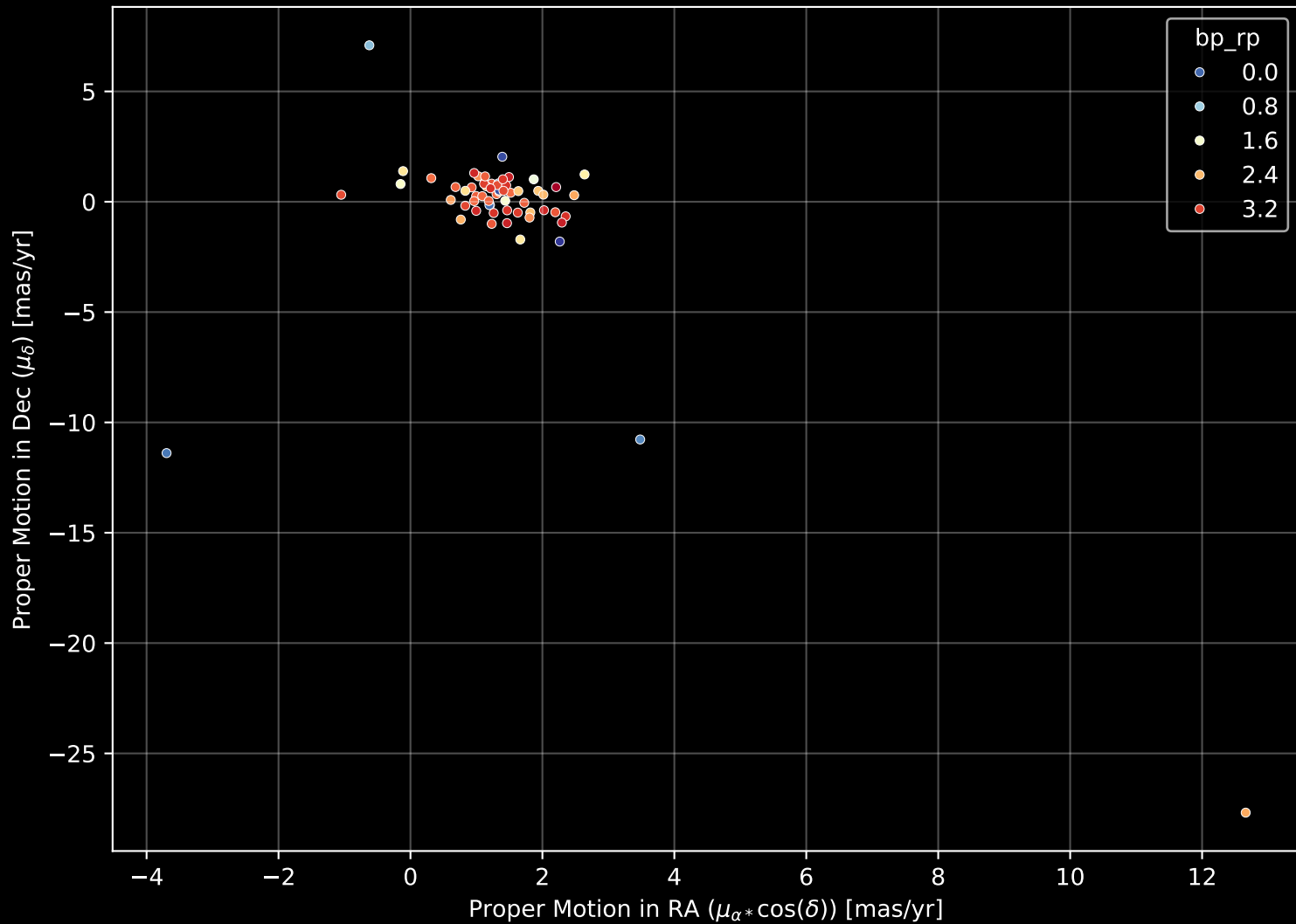
APOGEE DR17 Field: [209-20-C] Proper Motion Diagram (n= 63)
